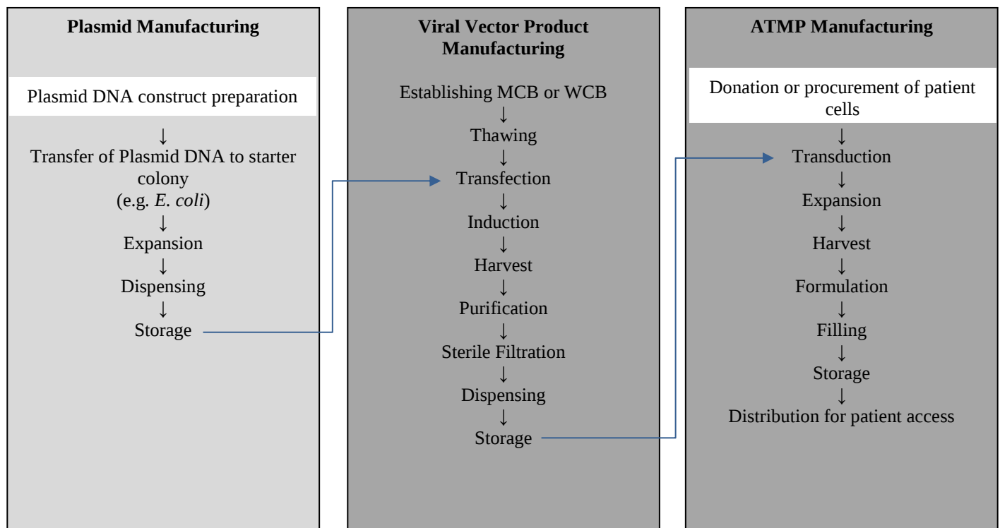
Figure 3: Example of autologous CAR-T therapy ATMP manufacturing
